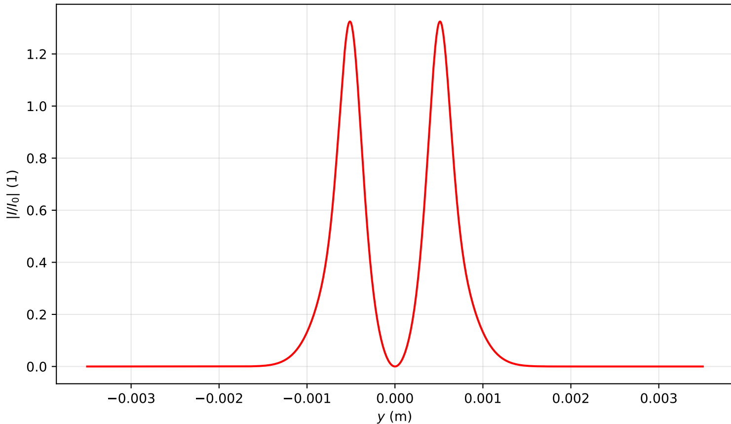
Intensity profile I(x=0, y, z=0.398)/I_0 , \text{Pin}=7.0\text{Pcr} , artificial time
